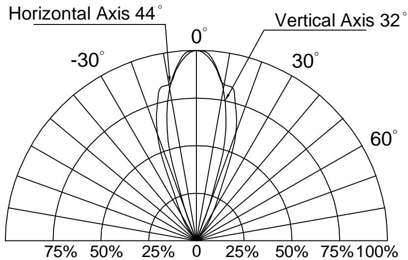
Radiation Angle(0.5):H 44 Degree/V 32 Degree
